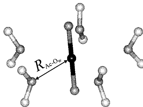
Figure 1. The pentagonal bipyramid geometry of \text{AcO}_2^{2+} \cdot 5\text{H}_2\text{O} ( \text{Ac} = \text{U, Pu} ).
