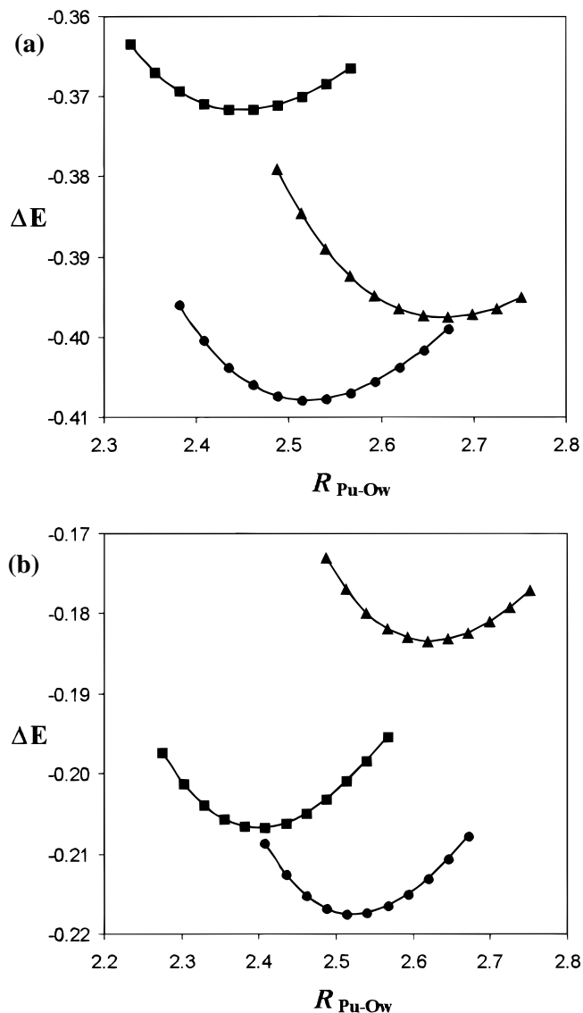
Figure 3. The dissociation energies, \Delta E , as a function of the plutonium–water oxygen distance, R_{\text{Pu-Ow}} , of the \text{PuO}_2^{2+} \cdot n\text{H}_2\text{O} complex in (a) the gas phase and (b) the liquid phase. Energies are in Hartree, distances in Å, and the three curves represent n = 4 (squares), n = 5 (circles), and n = 6 (triangles).
