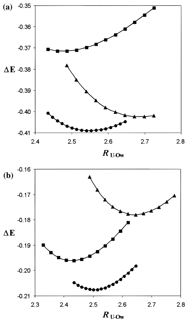
Figure 2. The dissociation energies, \Delta E , as a function of the uranium–water oxygen distance, R_{\text{U-Ow}} , of the \text{UO}_2^{2+} \cdot n\text{H}_2\text{O} complex in (a) the gas phase and (b) the liquid phase. Energies are in Hartree, distances in Å, and the three curves represent n = 4 (squares), n = 5 (circles), and n = 6 (triangles).
